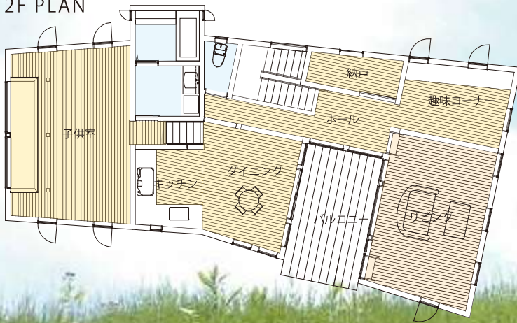
2F PLAN
